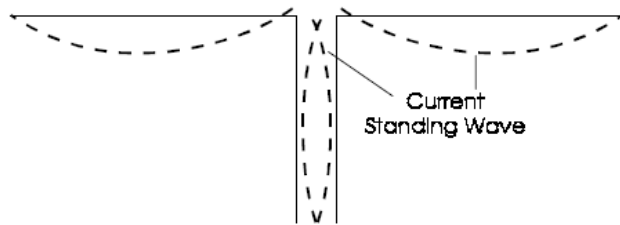
Current Distribution on 30 Meters
