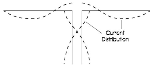
Current Distribution on 20 Meters
