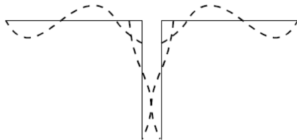
Current Distribution on 12 Meters
